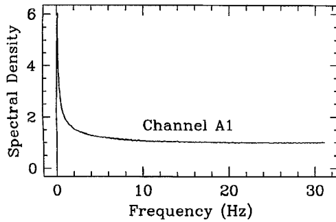
Fig. 3. Spectral density of the power fluctuations of the A1 channel of the radiometer obtained with the radiometer configured as in Fig. 2.
