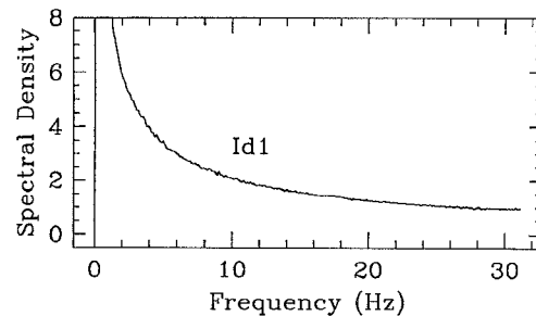
Fig. 8. Spectral density of the drain current fluctuations of the first stage of the HEMT amplifier obtained with the gate and drain voltages held constant.
