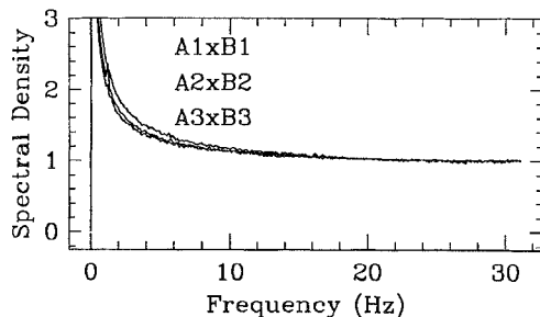
Fig. 6 Spectral density of the power fluctuations obtained from the cross-correlations between the same frequency bands of the two radiometer channels, A1 \times B1 , A2 \times B2 , and A3 \times B3 .
