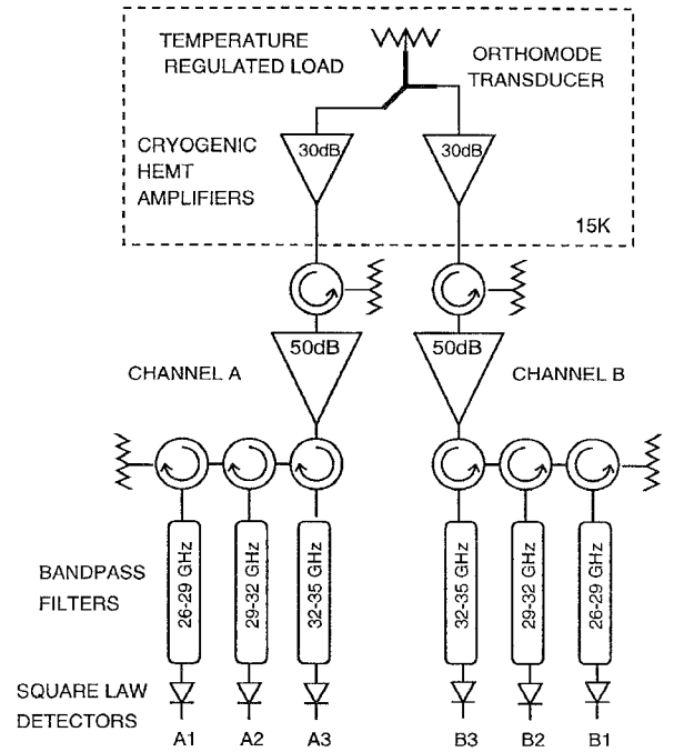
Fig. 2. Detailed block diagram of the radiometer employed in these measurements. The items enclosed in the dashed box were cooled to \sim 15 K by a closed cycle helium refrigerator.
