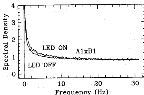
Fig. 10. Spectral density of power fluctuations as obtained from the cross-correlations A1 \times B1 with the light-emitting-diode which illuminates the HEMT's ON (upper) and OFF (lower).
